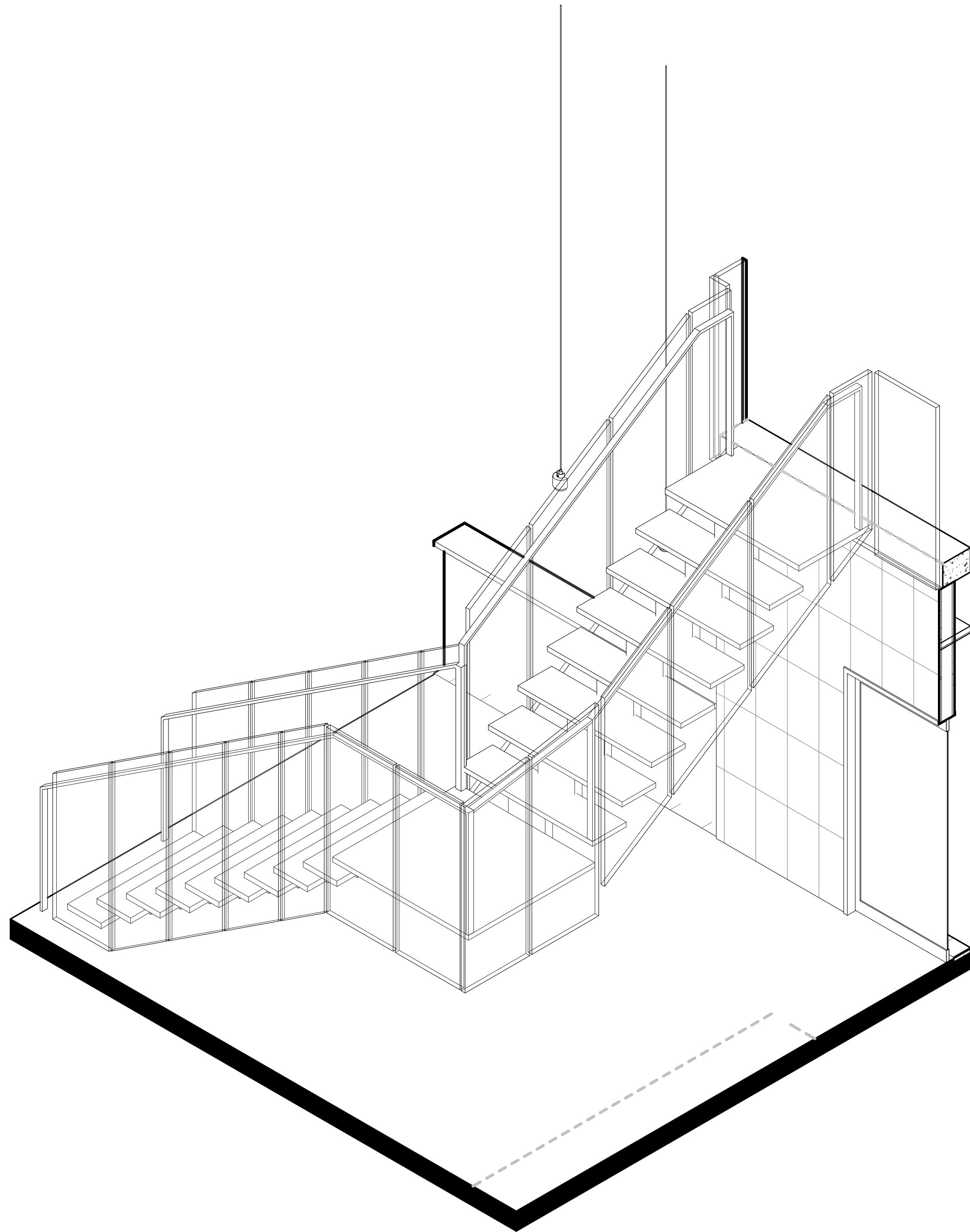
2 STAIR Isometric 2
