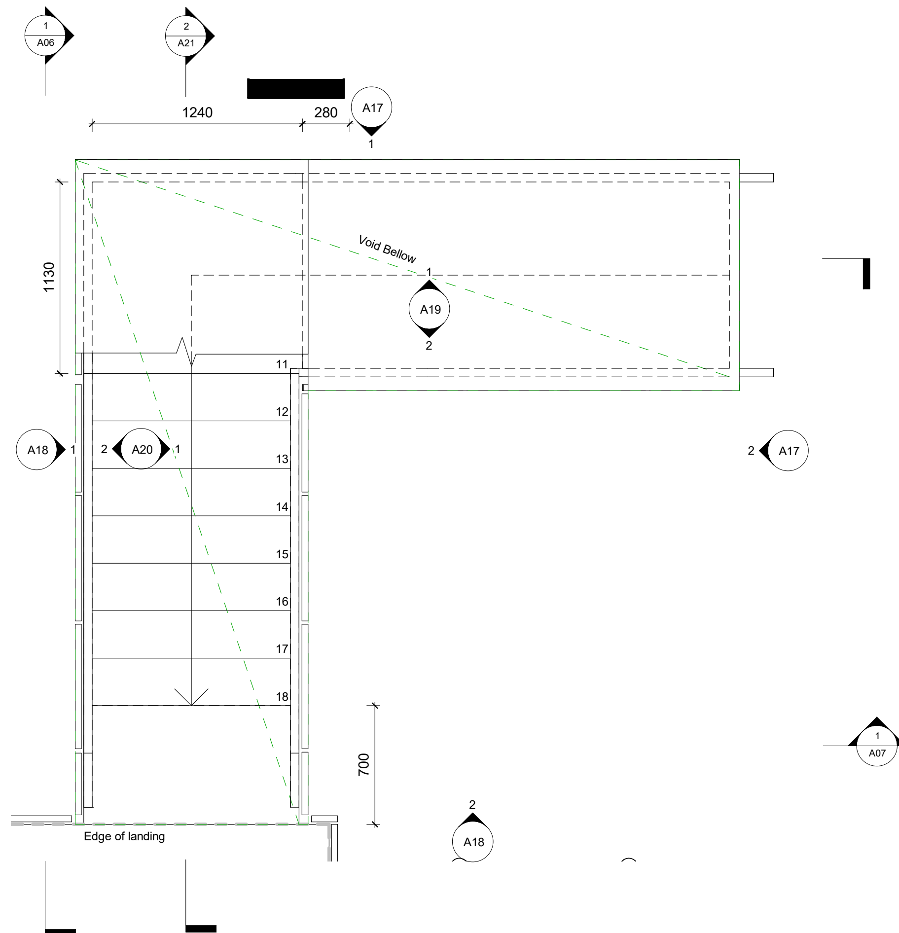
2 STAIR Detail Plan Upper 1 : 20
