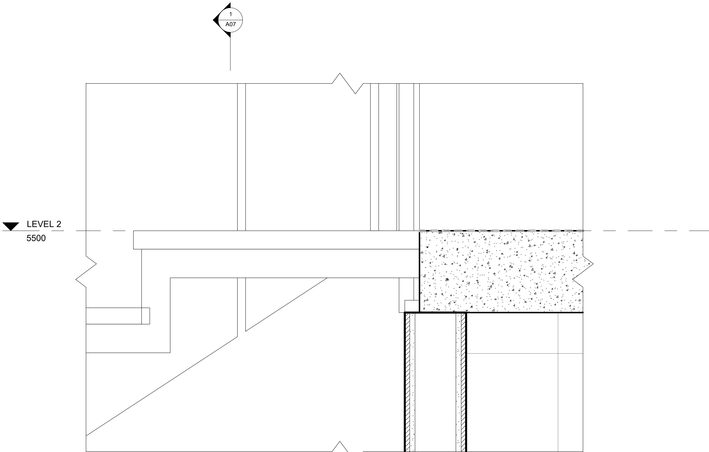
1 STAIR Tread 1:5
