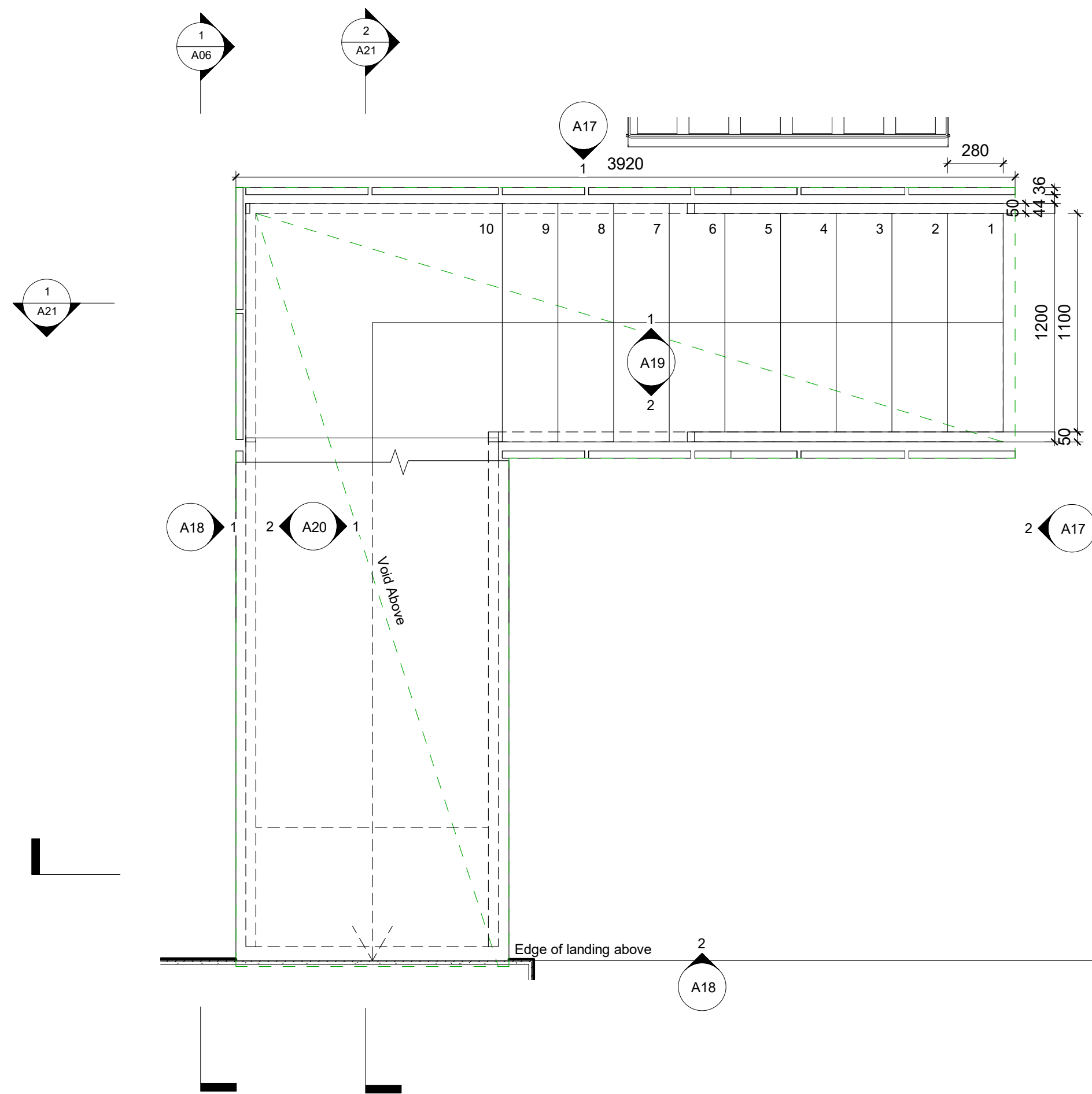
1 STAIR Detail Plan Lower 1 : 20
