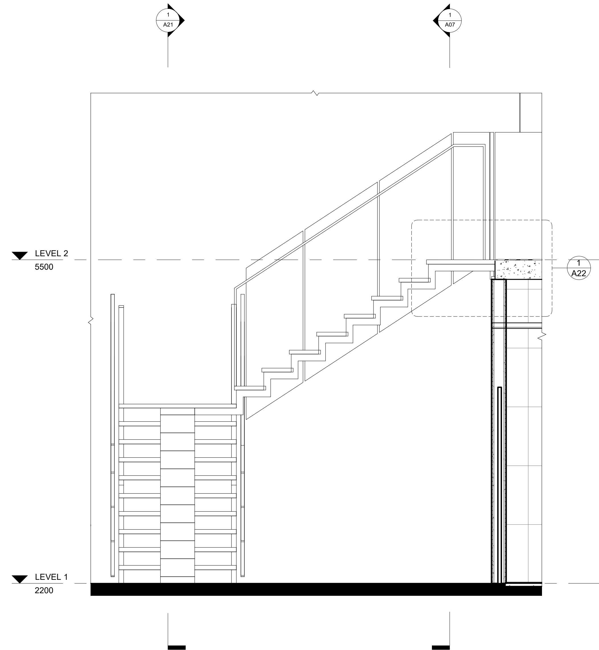
2 STAIR Section 1 1:20
