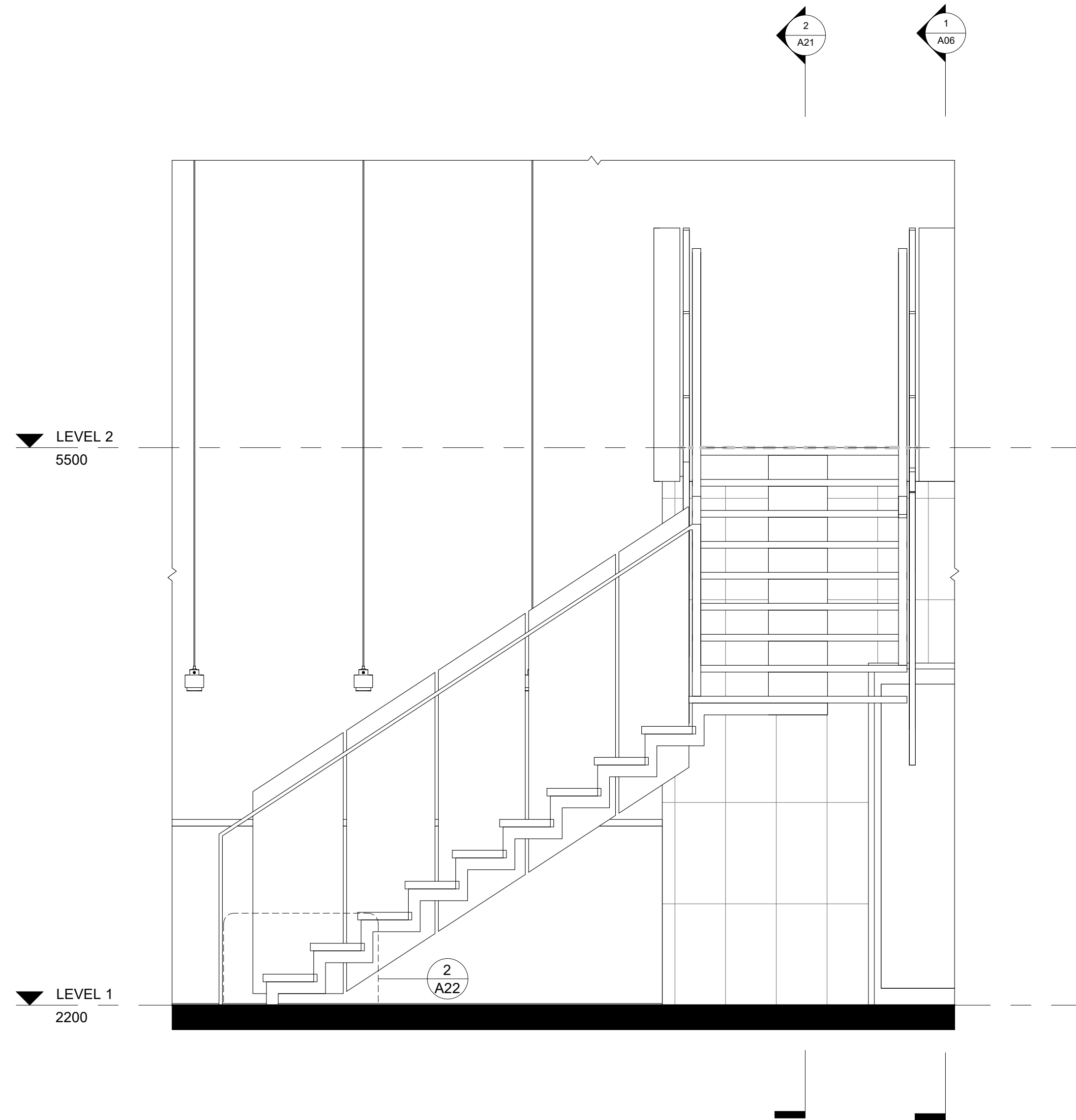
1 STAIR Section 2 1:20
